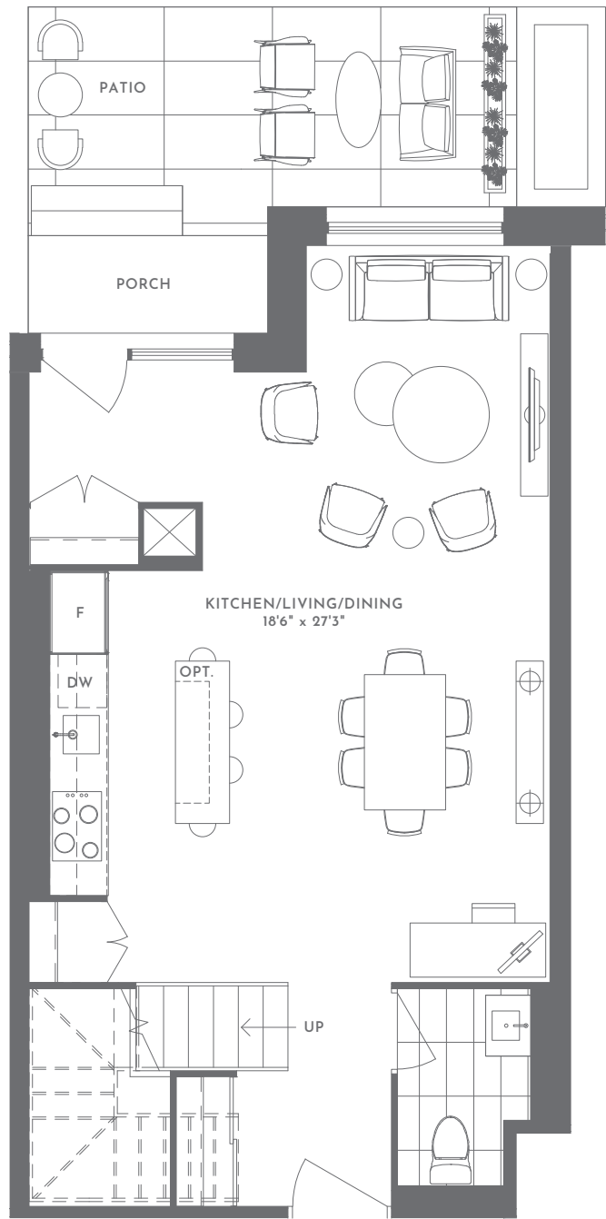
LEVEL 1
