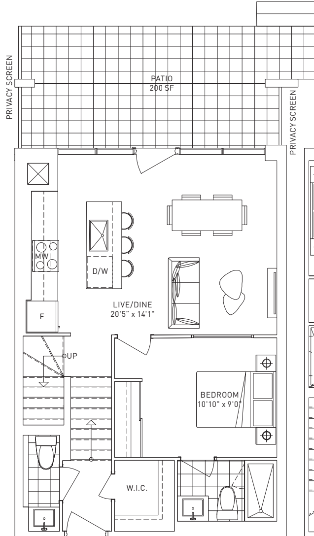
LOWER FLOOR
