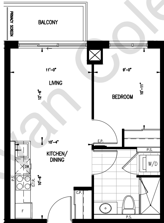
UNITS 202, 203, 302, 303, 324, 402, 403, 424, 502, 503, 524, 602, 603, 621, 702, 703, 721
