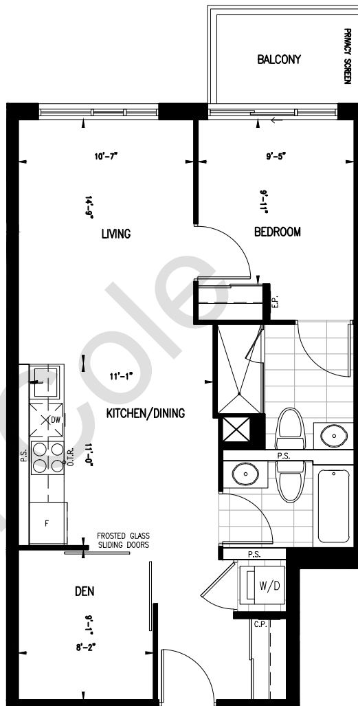
UNITS 427, 527, 624, 724, 817, 919, 1019, 1115, 1215, 1414, LPH14
