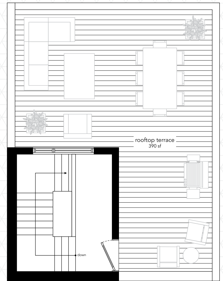
Third Floor
